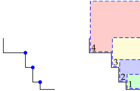
Figure 3.7: A staircase with T = 3 teeth marked by discs (Left). It has T + 1 = 4 corners and can be covered by 4 squares (Right).
