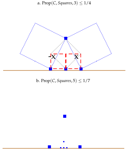
Figure 3.5: Impossibility result for 3 agents on a half-plane. See Claims 3.3.5-3.3.6.
