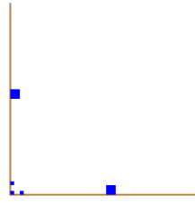
Figure 3.3: Impossibility results in a quarter-plane cake.
