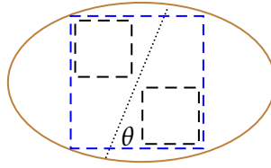
Figure 4.13: Dividing a convex R -fat cake to two people. The cake (the ellipse) is divided by a rotating knife (dotted line) to two 2R -fat convex pieces. This is a convex variant of Figure 4.6.
