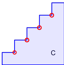
Figure 5.2: A rectilinear polygon with 4 reflex vertexes (circled).
