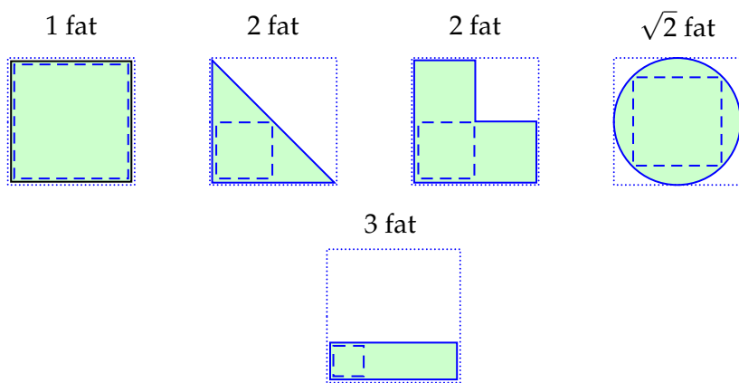
Figure 2.1: Fatness of several 2-dimensional geometric shapes. The dashed square is the largest contained cube; the dotted square is the smallest containing parallel cube. The shape is R -fat if the ratio of the side-lengths of these squares is at most R .
