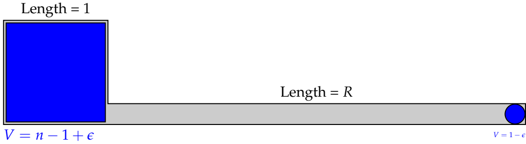
Figure 4.10: A fat cake in which every proportional division must use slim pieces. See Lemma 4.5.8.
