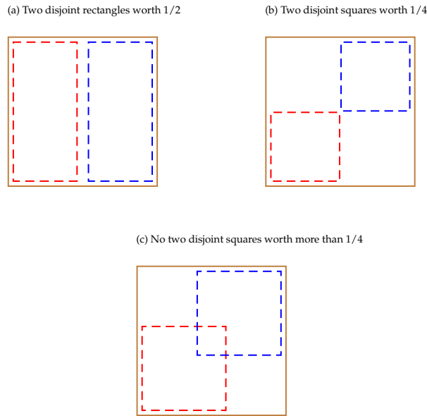
Figure 3.1: With geometric constraints, a proportional allocation might not exist.
