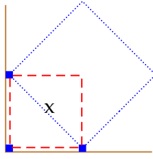
Figure 3.3: Impossibility results in a quarter-plane cake.
