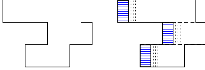
Figure 4.4: (a) A cake made of a union of 3 disjoint rectangles. (b) Three knife functions, each having a geometric loss of at most 4, proving that \text{PropEF}(C, \text{rectangles}, 2) \geq 1/4 .
