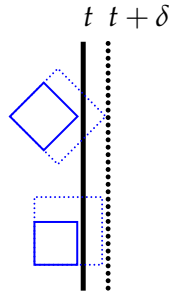
Figure 4.11: Square-continuity of the knife-function defined in Lemma 4.A.7. The solid line describes the knife location at time t ; the dotted line describes its location at time t + \delta . The dotted squares are squares contained in H(t + \delta) ; the solid squares are their predecessors in H(t) . At the bottom, the side-length of the solid square is smaller than the dotted square by exactly \delta . At the top, the side-length of the solid square is smaller than the dotted square by less than \delta .
